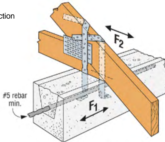
Typical Installation with Two METAs
