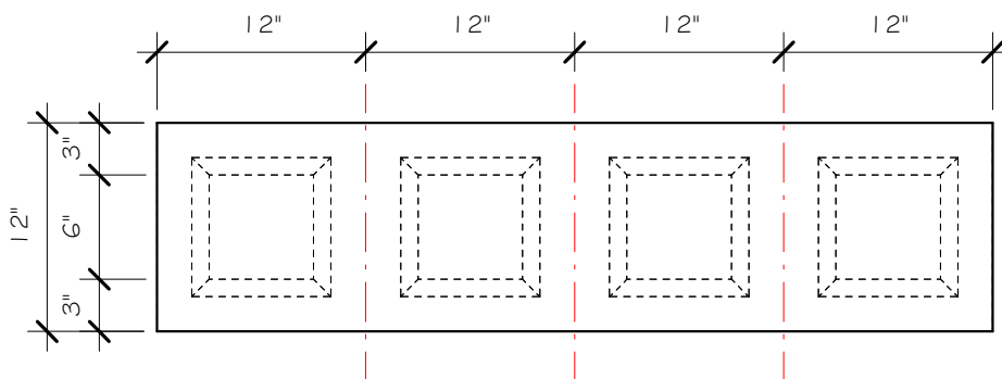
FRONT (WIREFRAME VIEW)
