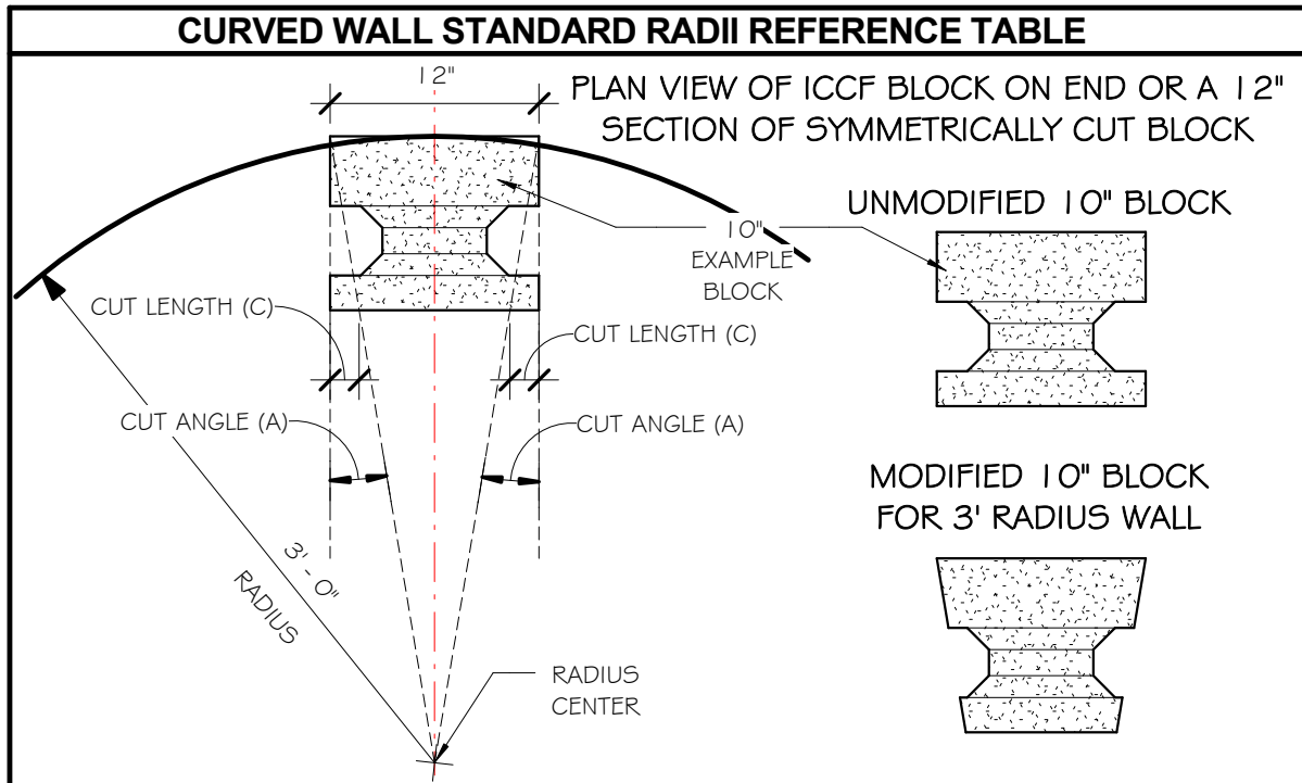
BLOCK CUTS FOR STANDARD RADII
